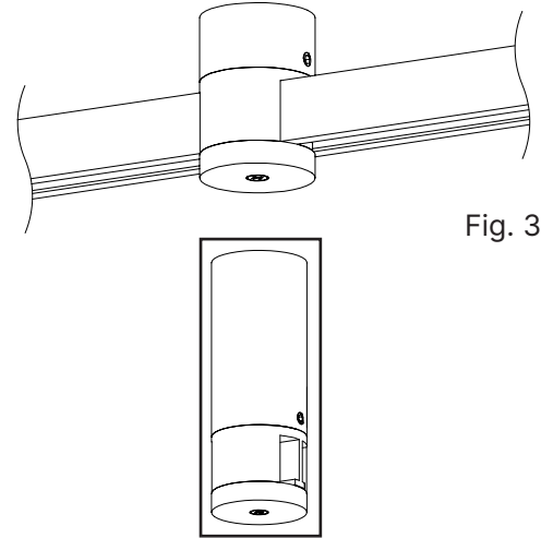
Applies to Ceiling Flush Mount Offset Support
